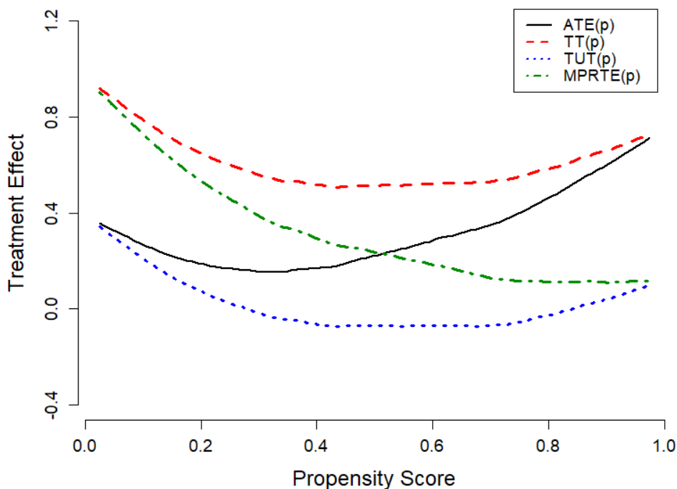
Figure 4: Heterogeneity in ATE, TT, TUT, and MPRTE(p) by Propensity Score based on Semiparametric Estimates of \widetilde{MTE}(p, u) .
